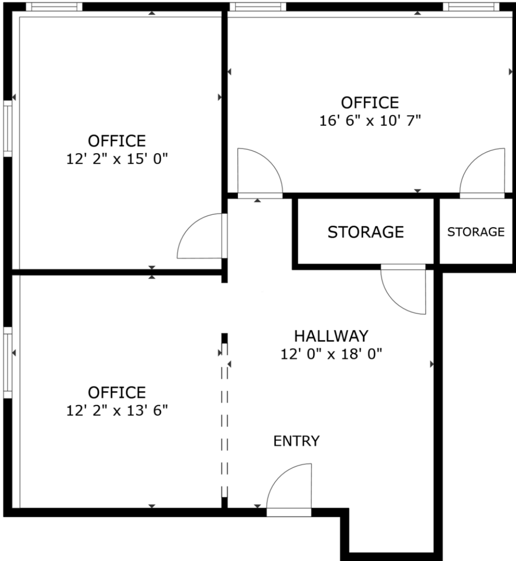
FLOOR PLAN
