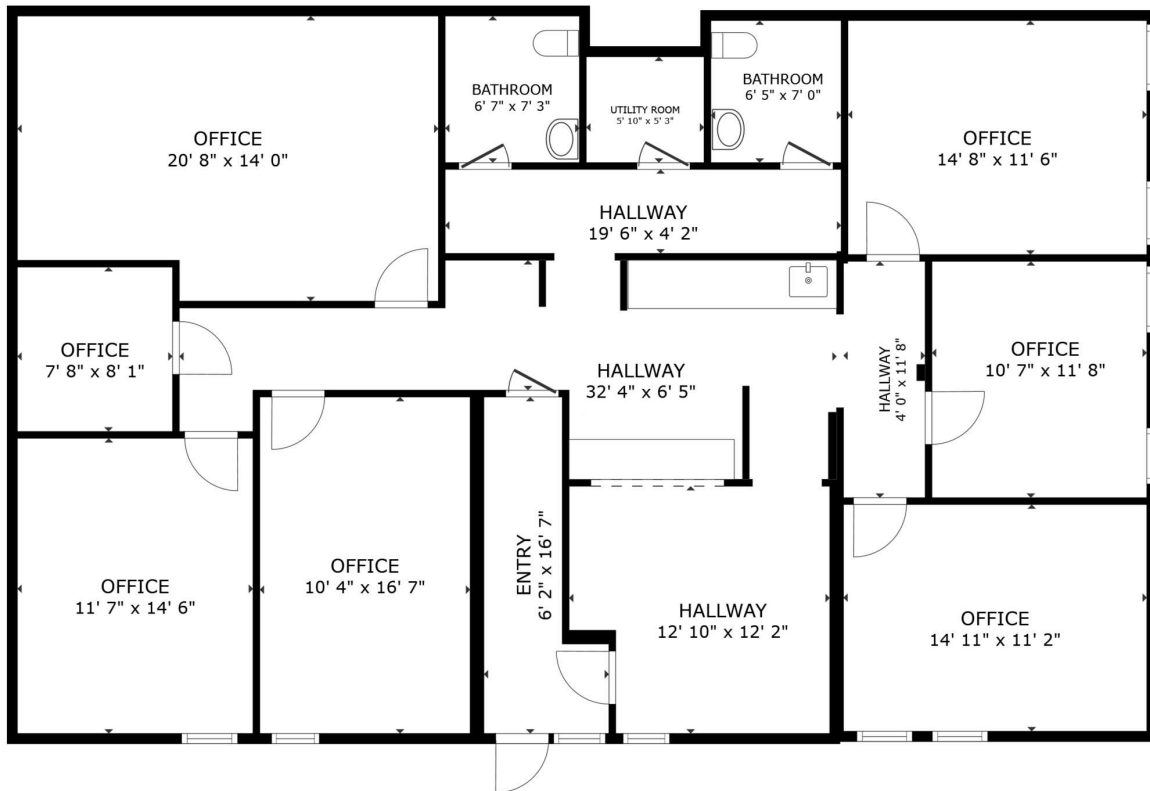
FLOOR PLAN
